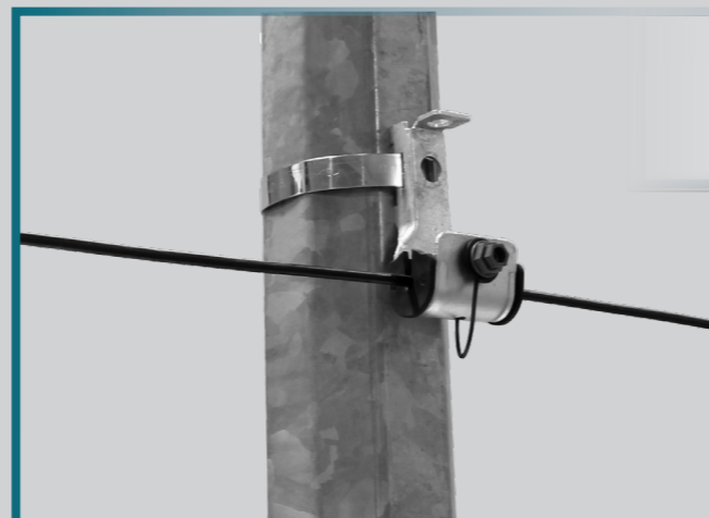
On a metal or composite pole with a band of strap
