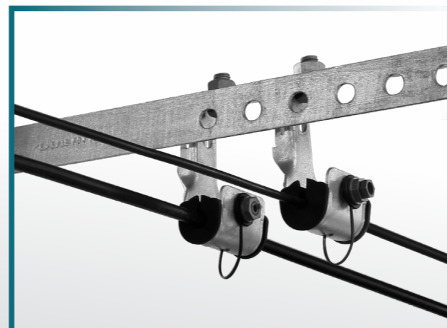
Under crossarm with assembling bolt
